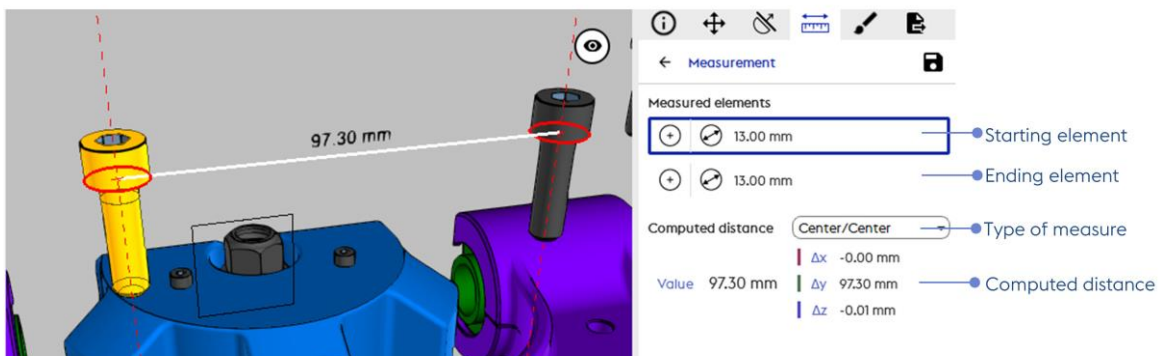
Measure distance - © Akka
